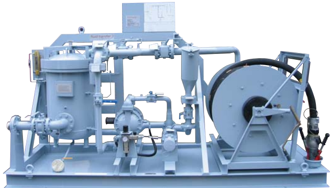
Helicopter Refuelling - Dispensing Skid
